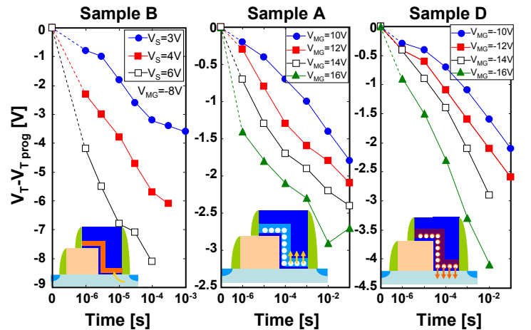
Figure 6. Erase characteristics of 30nm memories with various erasing mechanisms: Hot Hole Injection (sample B: Si 3 N 4 ), FN through top dielectric (sample A: Si-ncs) and FN through bottom dielectric (sample D: Si-ncs with high-k top oxide).
