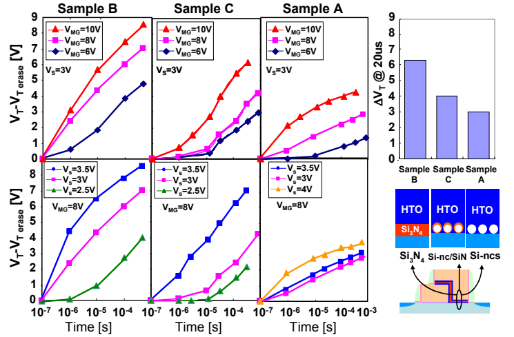
Figure 5. Left: Program characteristics in Source Side Injection mode of sample B (Si 3 N 4 ), sample C (Si-nc/SiN), sample A (Si-nc) with 30nm memory electrical gate length, for various programming V_{MG} and V_S . Right: Memory windows of Si-nc, Si-nc/SiN and Si 3 N 4 split-gate charge trap memories for same programming conditions ( V_{GM}=10V , V_S=3V , t_w=20\mu s ).
