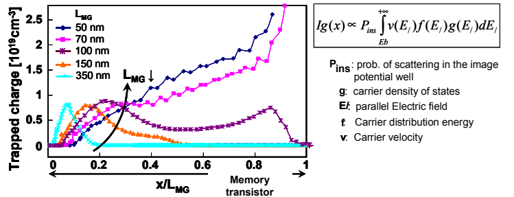
Figure 11. Simulated trapped charge in Si 3 N 4 (Fiegna model) during Source Side Injection programming operation for various gate lengths.
