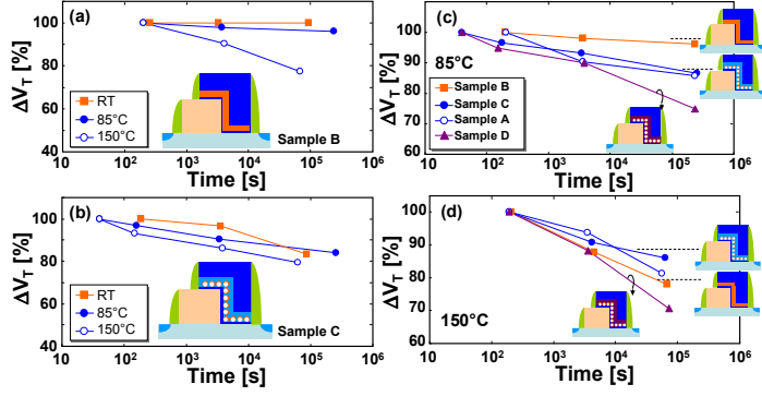
Figure 7. (a, b): Retention characteristics for various temperature for Si 3 N 4 (sample B) and Si-nc / SiN (sample C) charge trapping layers. (c, d): Comparison of retention characteristics at 85°C and 150°C of split-gate charge trap memories with various gate stacks.
