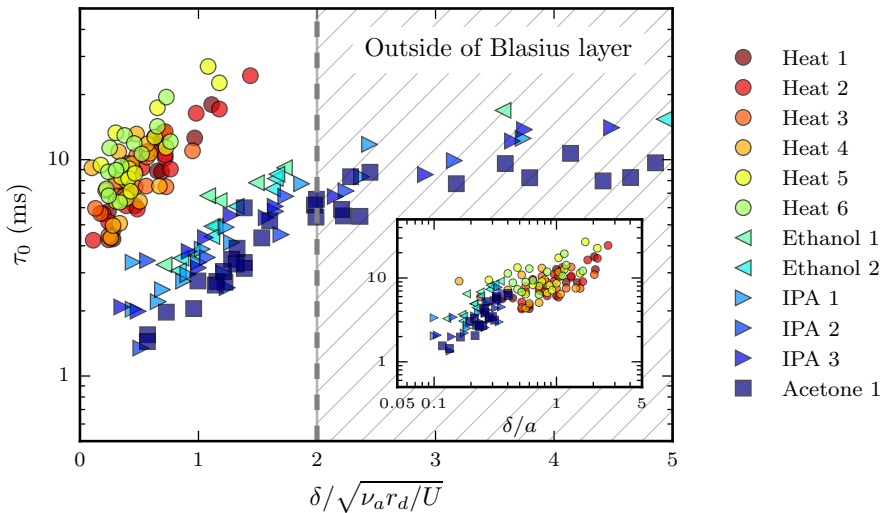
FIGURE 16. Instability timescale \tau_0 measured for different sollicitations, plotted versus the distance from the perturbation to the sheet \delta , scaled by the thickness of the Blasius boundary layer. The diverse runs correspond to different film velocities when the perturbation is chemical, or decreasing the temperature of the tip from 450^\circ\text{C} (Heat 1) to 200^\circ\text{C} (Heat 6) by steps of 50^\circ\text{C} , with no noticeable influence. In insert, \tau_0 is plotted against \delta/a , with a the size of the perturbation, for data inside the boundary layer ( \delta/\sqrt{\nu_a r_d/U} < 2 ).
