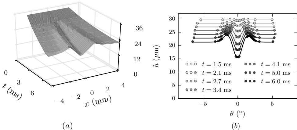
FIGURE 13. Film thickness. a) Interpolated thickness field. b) Transverse thickness profiles for different times (distances) after the perturbation. Experimental data (points) are plotted along with a the prediction in equation (4.7) (solid line) with r_d = 3.3 cm, with \alpha = 0.8 \pm 0.1^\circ and \tau_0 = 6.5 ms giving Pe = 3 \times 10^4 . Ethanol drop, water film, U = 3.2 m s ^{-1} , h = 34 \mu m.
