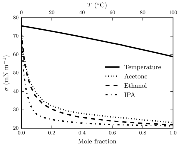
FIGURE 3. Surface tension dependences of isopropyl alcohol (IPA), ethanol (Vazquez et al. 1995) and acetone (Enders et al. 2007) solutions on their mole fraction in water. Dependence of water surface tension on temperature T (Vargaftik et al. 1983).
