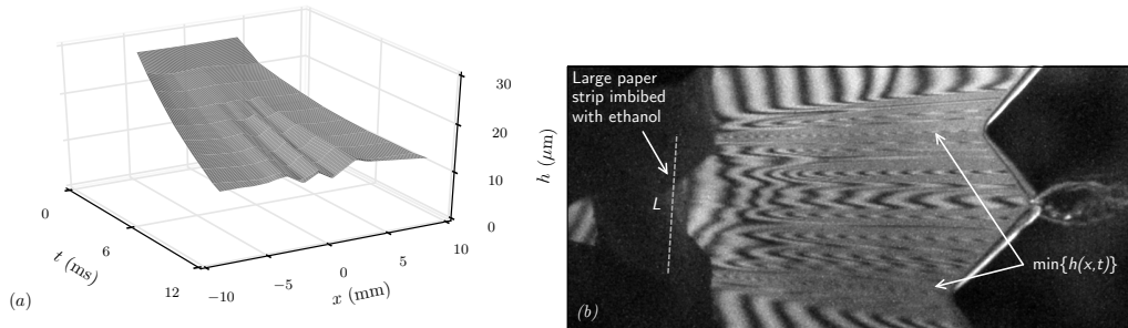
FIGURE 18. Broad support of surface tension deficit. a) Measured thickness field for an ethanol source of size L = 4.6 mm. The thickness decreases at the edges of the source. b) Sheet rim double retraction, with an even larger perturbation L = 10 mm. Two cusps appear, signatures of the two decoupled thickness decreases.
