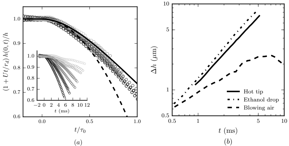
FIGURE 14. a) Film minimal thickness h(0, t) as a function of time t : time is rescaled by \tau_0 in the main graph, original time dependences are in the insert. From lightgray to black, \tau_0 equals successively 24.9; 16.9; 14.3; 10.9; 10.7; 8.7; 6.9; 6.7 and 5.1 ms. The solid line is expression 4.9 and the dashed line its short time expansion. b) Thickness difference \Delta h between film thinnest and thickest points as a function of time, for 3 different local perturbations: hot tip ( \tau_0 = 5.6 ms), ethanol drop ( \tau_0 = 6.5 ms) and blowing air on the film.
