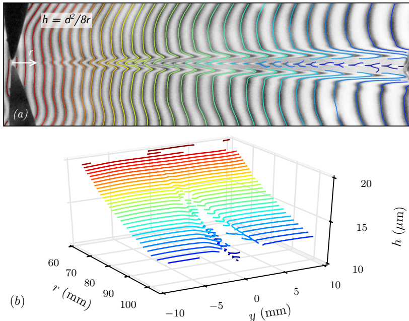
FIGURE 5. Thickness measurement technique. a) Typical interferometric picture. Each dark fringe is a line of iso-thickness, separating from the following by a constant \Delta h \approx 0.25 \mu\text{m} . A reference is made where the film is unperturbed. b) Iso-thickness ridges are plotted in 3D.
