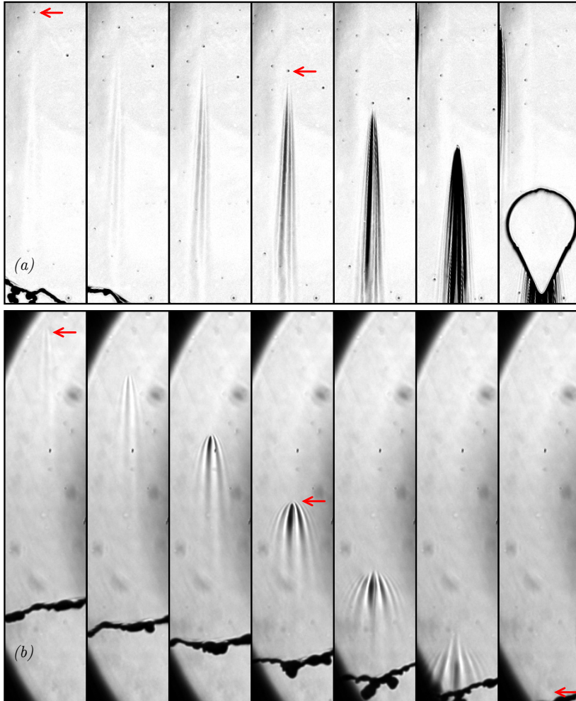
FIGURE 8. Ethanol droplets approaching a 10\ \mu\text{m} thick film falling downwards ( U = 4.7\ \text{m s}^{-1} ). a) Pictures are 12\ \text{mm} wide, recorded every \Delta t = 4\ \text{ms} . Note the uneven hole opening shape after the droplet pierces the film. b) Pictures are 9.3\ \text{mm} wide, \Delta t = 2\ \text{ms} . The tiny droplet rebounds on the film and modifies the thickness field, but does not puncture it (see also figure 1).
