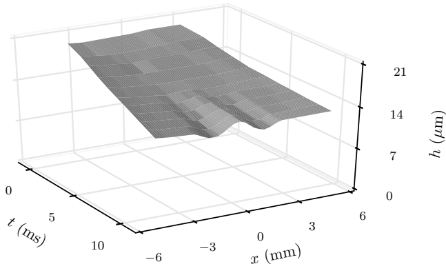
FIGURE 17. Measured thickness field for an excess of surface tension in the dirty spot (water drop close to an ethanol sheet, a = 1.5 mm, r_d = 56 mm giving \alpha = 1.5^\circ ). The interstitial liquid is now concentrated at the center of the spot, instead of being expelled at its periphery (see figure 13 for comparison).
