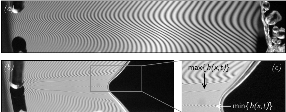
FIGURE 15. Sheet rim retraction. a) Unperturbed sheet, flowing from left to right. The sheet ends up in a corrugated rim. Picture is 48 mm wide. b) Sheet perturbed by an alcohol drop decreasing locally its surface tension: the rim retracts and gets smooth. c) Close-up view of the smooth rim.
