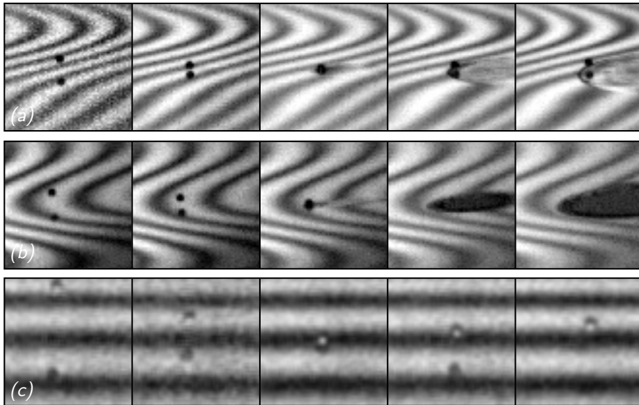
FIGURE 6. a) Water or b) ethanol droplet ( 200\ \mu\text{m} in diameter) falling on a moving water film ( U = 3.5\ \text{m}\cdot\text{s}^{-1} ) with thickness h = 18\ \mu\text{m} . Pictures are 3.3\ \text{mm} wide, recorded every \Delta t = 250\ \mu\text{s} . a) The water droplet rebounds, when b) the ethanol droplet pierces the film. c) Ethanol droplet ( 150\ \mu\text{m} in diameter) falling on a static soap film with thickness h = 5\ \mu\text{m} , and rebounding. Pictures are 1.1\ \text{mm} wide, recorded every \Delta t = 1\ \text{ms} .
