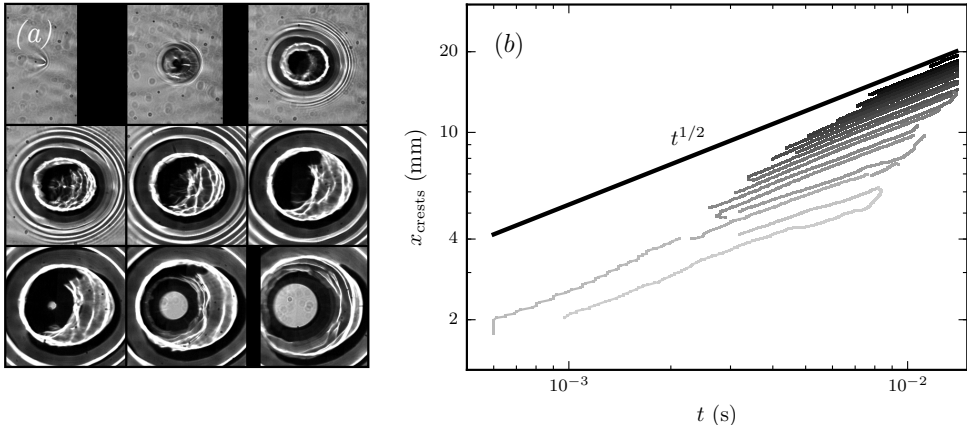
FIGURE 10. a) Wave pattern (and film rupture) generated by a droplet of ethanol ( a = 100 \mu\text{m} ) landing on a thick water film h = 250 \mu\text{m} . Pictures are 8.6 mm wide, recorded every 800 \mu\text{s} , reading from left to right, top to bottom. b) Wave crests are tracked along time and their location x_{\text{crests}} is plotted in logarithmic scale.
