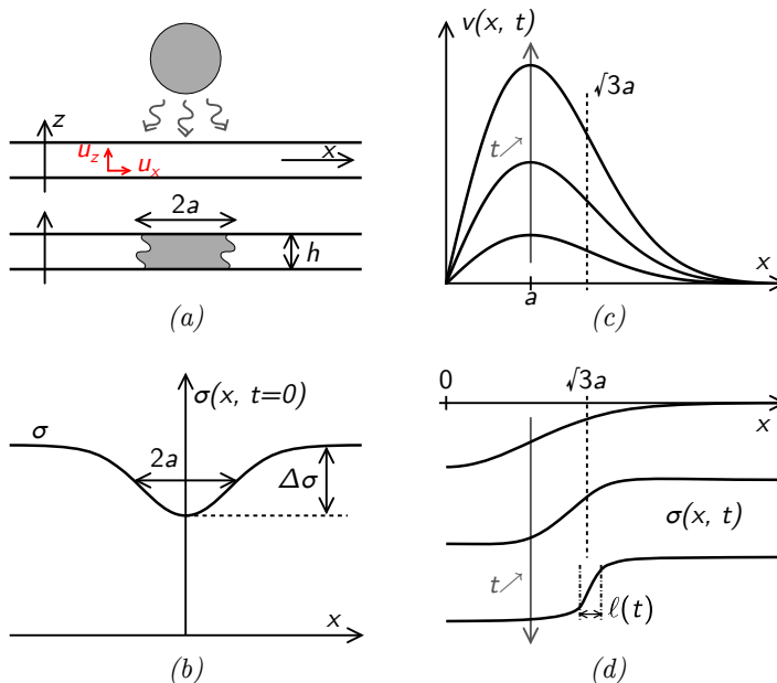
FIGURE 9. Sketch of the mechanism. a) A liquid film with thickness h being contaminated over a size 2a . b) Initial profile of the liquid surface tension. c) Induced displacement field v(x, t) along the film for increasing times t . d) Surface tension profiles for increasing times illustrating the existence of a plateau at \sigma - \Delta\sigma around x = 0 , and an steepening front around x = a\sqrt{3} of decreasing width \ell(t) .
