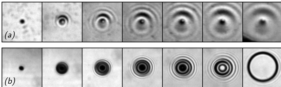
FIGURE 7. a) Water droplet falling on a moving water film ( U = 3.8\ \text{m}\cdot\text{s}^{-1} ) with thickness h = 14\ \mu\text{m} , and generating capillary waves. Pictures are 3.6\ \text{mm} wide, recorded every 700\ \mu\text{s} . b) Ethanol droplet falling on a moving water film ( U = 3.9\ \text{m}\cdot\text{s}^{-1} ) with thickness h = 13\ \mu\text{m} , and piercing it. Pictures are 5.8\ \text{mm} wide, recorded every 500\ \mu\text{s} .
