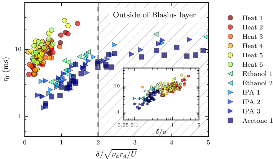
FIGURE 16. Instability timescale \tau_0 measured for different solicitations, plotted versus the distance from the perturbation to the sheet \delta , scaled by the thickness of the Blasius boundary layer. The diverse runs correspond to different film velocities when the perturbation is chemical, or decreasing the temperature of the tip from 450^\circ\text{C} (Heat 1) to 200^\circ\text{C} (Heat 6) by steps of 50^\circ\text{C} , with no noticeable influence. In insert, \tau_0 is plotted against \delta/a , with a the size of the perturbation, for data inside the boundary layer ( \delta/\sqrt{\nu_a r_d/U} < 2 ).
