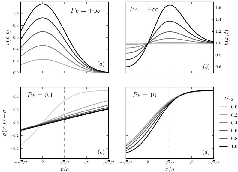
FIGURE 19. Time evolution of an initial step of surface tension of width a , for different Péclet numbers. Graphs are centered around x = a/\sqrt{2} , where compression is maximal. a) Interstitial velocity and b) film thickness for Pe = +\infty (or equivalently short times t/\tau_0 \ll 1 ). c-d) Surface tension profiles at successive times, for two finite Péclet numbers.
