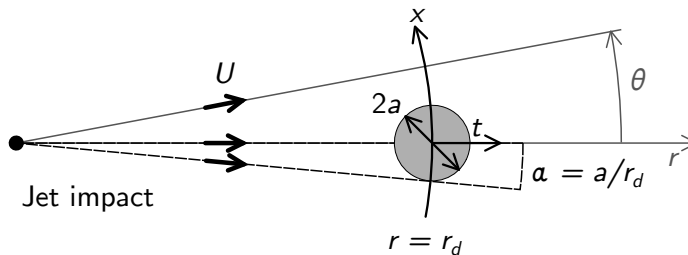
FIGURE 11. Geometrical transform of the natural (\theta, r) coordinates of the circular Savart sheet into (x, t) the coordinates of the mechanism.
