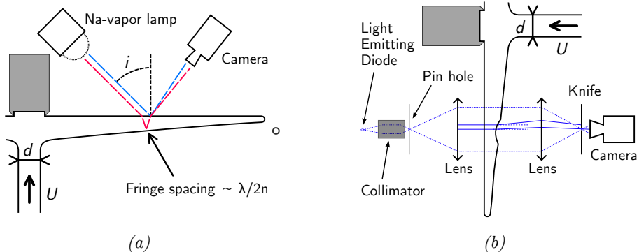
FIGURE 4. Visualisation techniques. (a) Interferometry: a sodium-vapor lamp inprints stripes on the sheet. Two consecutive fringes are separated by a constant thickness jump \Delta h = \lambda/2n \cos i_r , with i_r the refracted angle inside the sheet. (b) Schlieren: modulations of the thickness of the sheet, located in the plane of observation, deviate parallel light as would do optical lenses.
