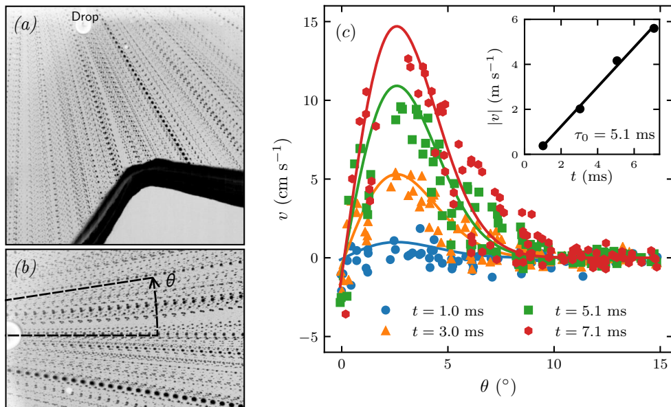
FIGURE 12. Velocity measurements of the interstitial flow. a) Superposition of 500 images grabbed at 3 kHz. b) Close-up view of the tracked particles in the correct coordinates system. Picture is 19 mm wide. c) Transverse velocity v as a function of the angle \theta to the drop, averaged around four successive times ( i.e. radii) from the drop location (for clarity, only positive angles are plotted). Acetone drop, water film ( U = 2.2 \text{ m s}^{-1} , Fr = 50 , h = 88 \text{ }\mu\text{m} ), r_d = 23 \text{ mm} , \alpha = 2.5^\circ , \tau_0 = 5.1 \text{ ms} , \Delta\sigma \simeq 3 \text{ mN m}^{-1} , Pe = 1.5 \times 10^5 . Inset: the amplitude |v| in the expression v = |v|\theta \exp(-\theta^2/2\alpha^2) (see equation (4.6)) is fitted to the experimental data and plotted versus time t for the corresponding successive times. The timescale \tau_0 reads directly from the slope r_d/\tau_0^2 .
