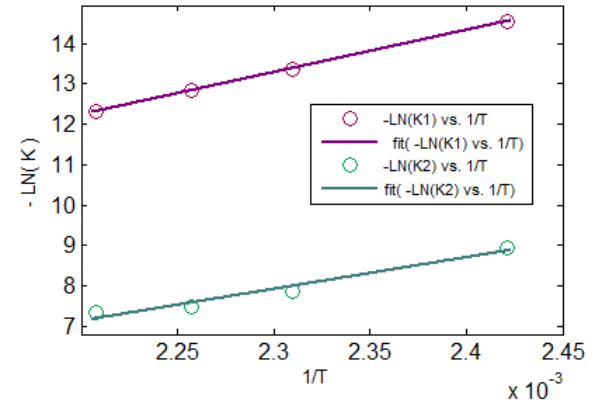
Figure 2: Reaction rate constants k1 and k2 .
