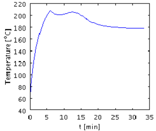
Figure 4: Temperature evolution with time at the center of the composite
