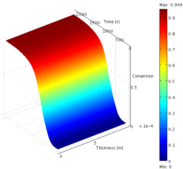
Figure 7: Degree of cure evolution with thickness and with time
