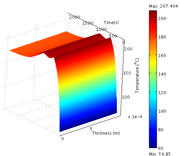
Figure 6: Temperature evolution with thickness and with time
