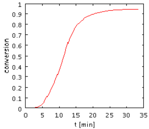
Figure 5: Degree of cure evolution with time at the center of the composite
