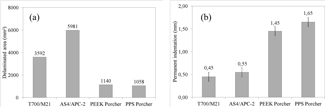
Figure 2. Delaminated areas (a) and permanent indentations (b) after impact
