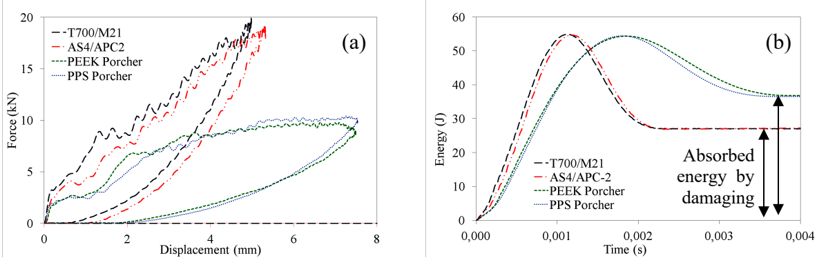
Figure 1. Curves of force versus displacement (a) and energy versus time (b) obtained experimentally
