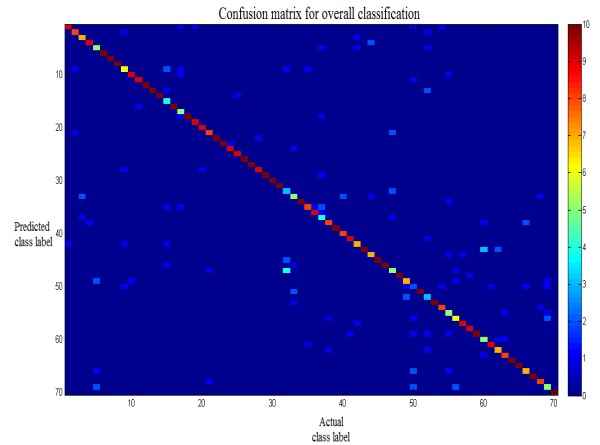
Figure 8: Confusion matrix for overall classification (MPEG-7 data set)
