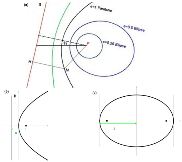
Figure 3: (a) Four conic with same focus and their directrix: ellipses ( e = 0.25 , e = 0.5 ), parabola ( e = 1 ) and hyperbola ( e = 2 ) with fixed focus F and directrix D . (b) Parabola according to angle \phi_1 = 180^\circ . (c) Ellipse according to angle \phi_2 = 0^\circ
