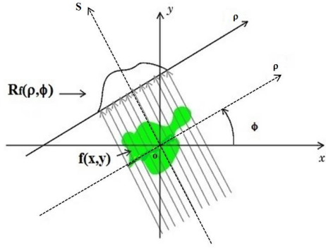
Figure 1: Geometry of the Radon transform over lines.
