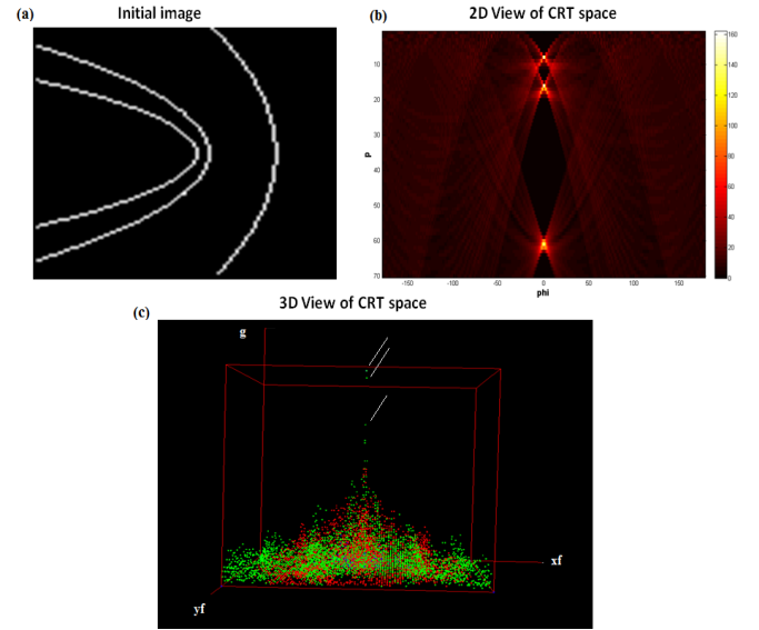
Figure 4: (a) Initial image where three parabolas are positioned at the center row. The result of the CRT on (a) is the (x_F, y_F, \rho, \phi, e) parameters space where (b) present 2D view of CRT space ( e = 1 , x_F = y_F = 0 ) and the coordinates of each of the peaks corresponds to the parameters (\phi, \rho) of the curves. \rho is the distance of focus to directrix and \phi is the orientation of parabola. (c) present 3D view of CRT space according to (x_F, y_F, R_c f((x_F, y_F, \rho, \phi, e))) where the color corresponds to the eccentricity e (blue: ellipse, green: parabola, red: hyperbola) and the peaks which have green color corresponds to parabolas.
