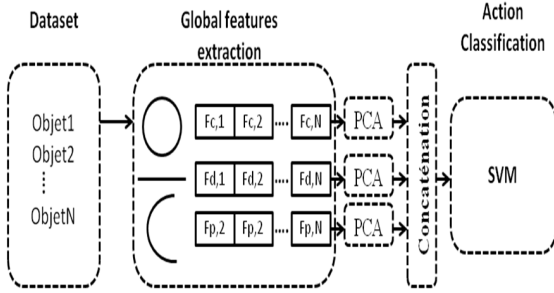
Figure 6: Architecture of proposed approach
