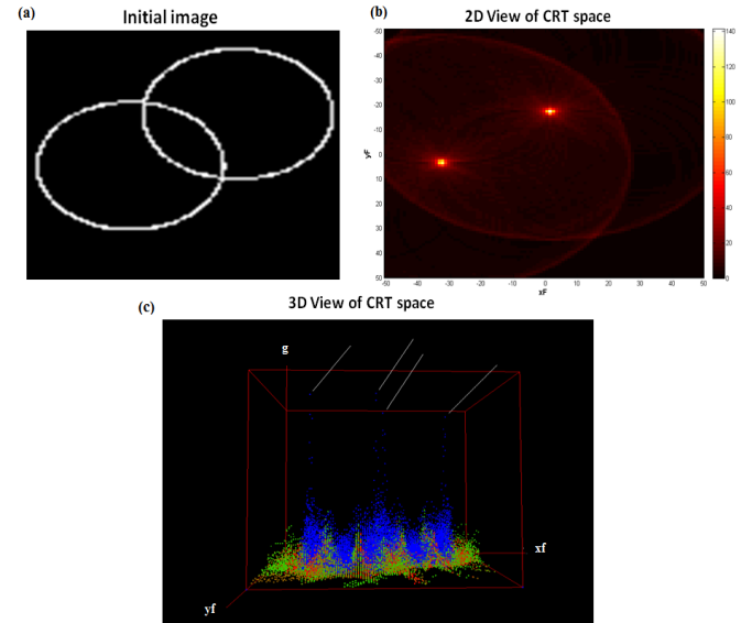
Figure 5: (a) Initial image where two ellipses are presented. (b) 2D view shows the peaks corresponding to the position of one focus for each ellipse. (c) The coordinates of each of the maximum value correspond to the parameters (x_F, y_F, R_c f((x_F, y_F, \rho, \phi, e))) of the four focus of ellipses according to (\phi = 0^\circ, e = 0.5, \rho = 22) . The peaks have blue color which corresponds to ellipses.
