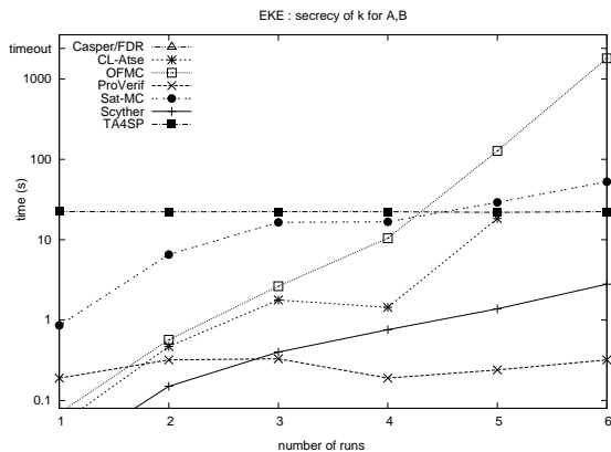
Fig. 4. Time efficiency comparison for EKE [7], secrecy
