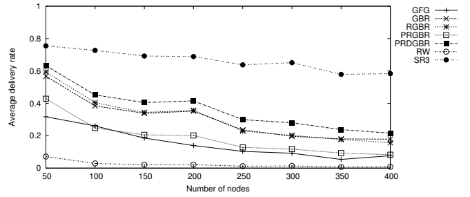
Fig. 1. Average delivery rate (30% of BH nodes, \bar{d} = 8 )
