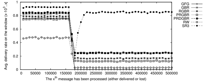
Fig. 8. Average delivery rate (5% of WH/BH, 5% of BH, n = 200 , \bar{\delta} = 8 )
