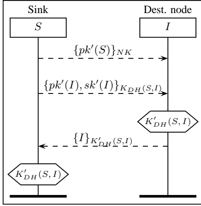
(a) Protocol RAKnka: S and I compute K'_{DH}(S, I) .
