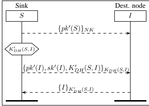
(b) Protocol RAKnkb: S computes K'_{DH}(S, I) and sends it to I .
