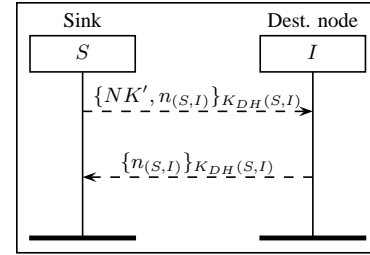
Figure 5: Protocol RNK: Renewing the Network Key.
