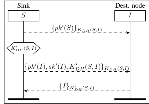
(b) Protocol RAKdhb: S computes K'_{DH}(S, I) and sends it to I .
