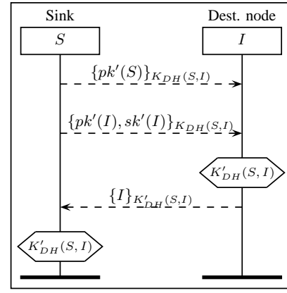
(a) Protocol RAKdha: S and I compute K'_{DH}(S, I) .
