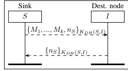
Figure 1: Protocol KR: Revocation of k malicious neighbor nodes of node I .
