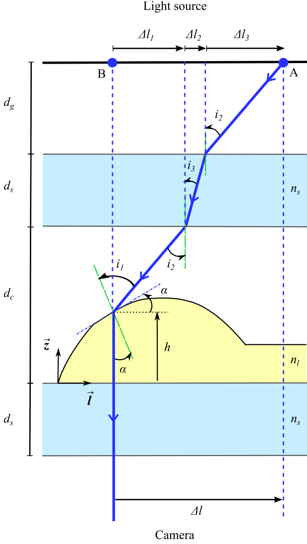
Fig. 3. Ray tracing in the plane (\mathbf{l}, z) orthogonal to the triple contact line and to the porthole plane. In reality, d_g is much larger than both d_s and d_c , and d_c = d_s .
