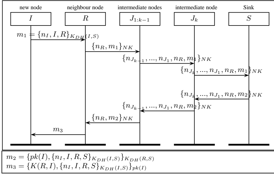
Fig. 6: IJS_{NK,dec/enc} : Proof by Induction.
