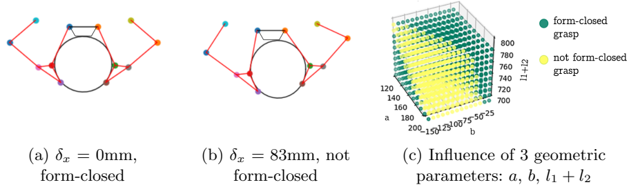
Fig. 5: Form-closure evolution.
