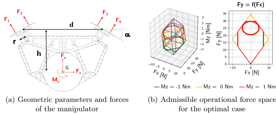
Fig. 3: Manipulability study
