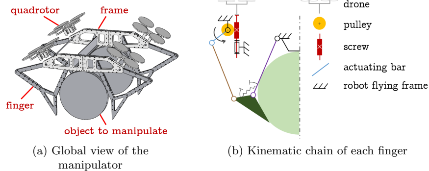
Fig. 1: Flying manipulator presentation
