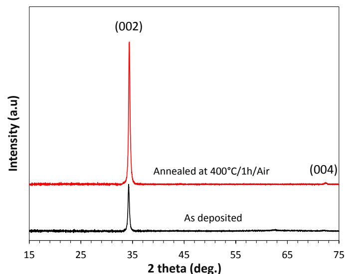
Figure 3. XRD pattern of a 100 nm ZnO:Ga film deposited on glass, before and after annealing under air at 400 \text{ }^\circ\text{C} .
