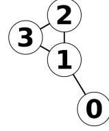
Fig. 1. The flower F_1 .
