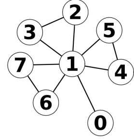
Fig. 5. The flower F_3 .
