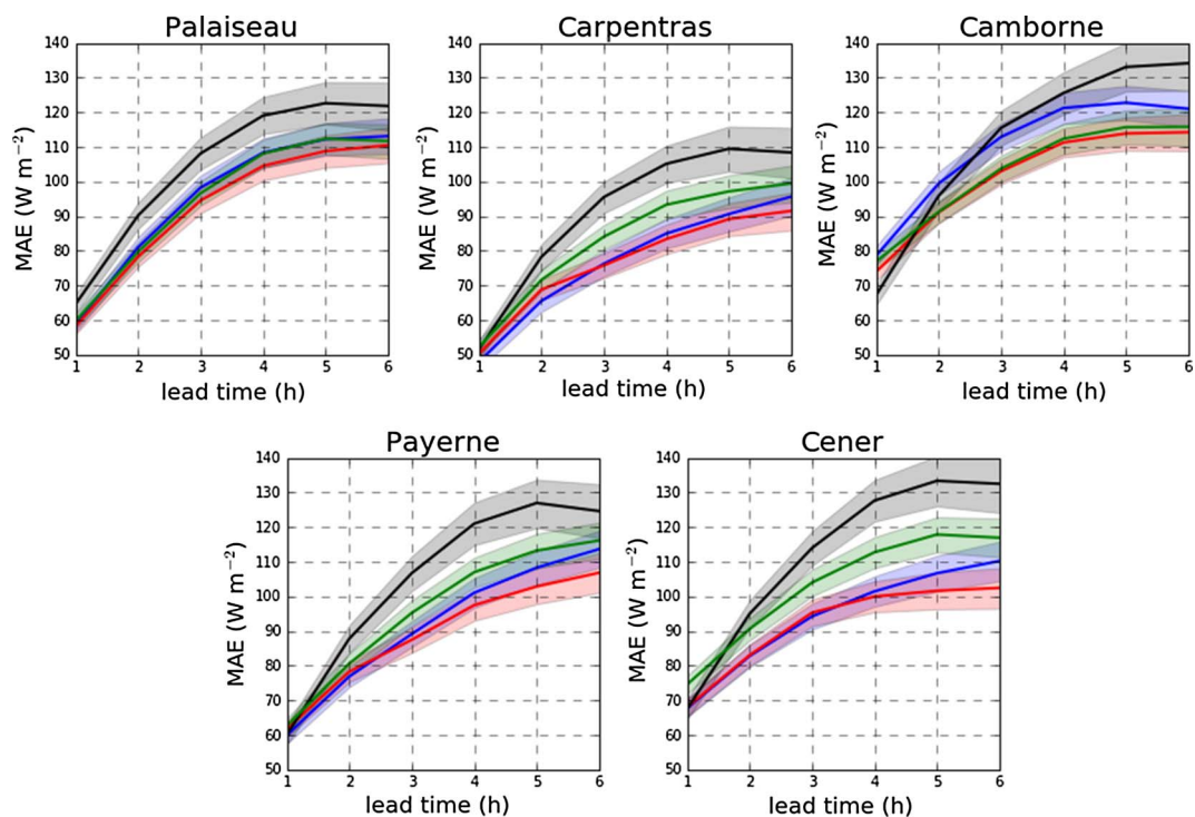
Fig. 10. Mean MAE and corresponding 95% bootstrap confidence interval as a function of lead time for the analog method (blue), the post-processed analog method (red), the persistence method (black), and the adaptive VAR(1) model (green). (For interpretation of the references to colour in this figure legend, the reader is referred to the web version of this article.)
