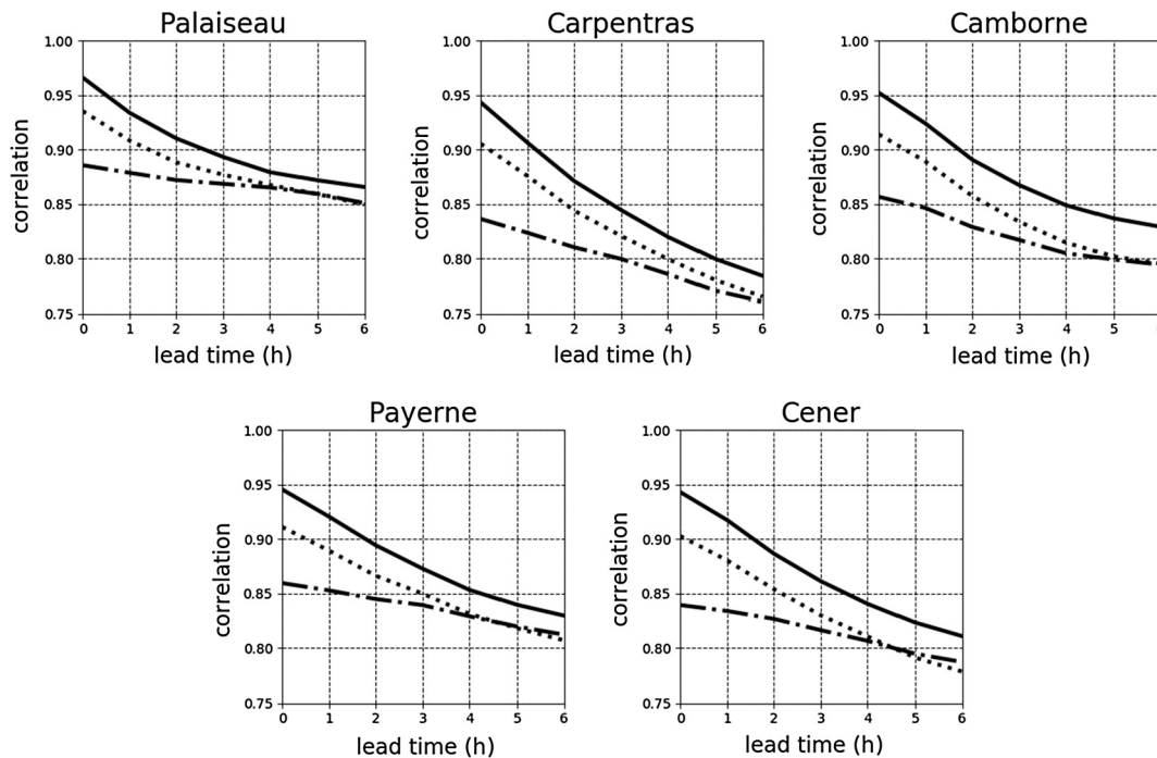
Fig. 5. Mean correlation over the test data set between current observations and best analog-successor for different lead times. Three strategies are studied: the best analog without translation (dotted-dashed), the best analog with translation (dotted) and the best translated analog with respect to the weights given in Eq. (7) (full line).
