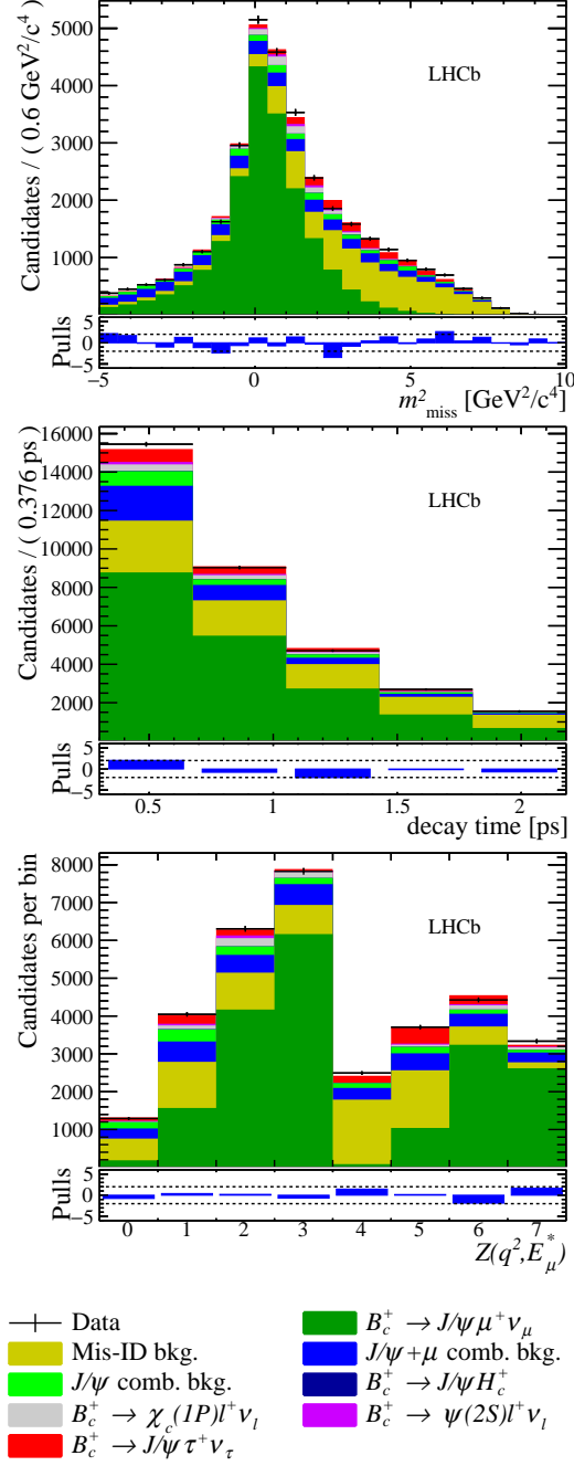
Figure 1: Distributions of (top) m^2_{\text{miss}} , (middle) decay time, and (bottom) Z of the signal data, overlaid with projections of the fit model with all normalization and shape parameters at their best-fit values. Below each panel differences between the data and fit are shown, normalized by the Poisson uncertainty in the data; the dashed lines are at the values \pm 2 .
