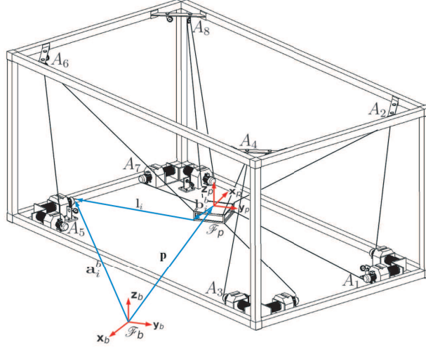
Fig. 1: Geometric description of a fully constrained CDPR
