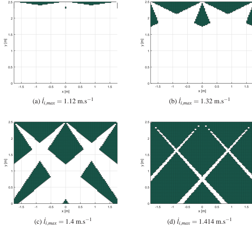
Fig. 6: TFW of the planar CDPR for four maximum cable velocity limits and for the RTS shown in Fig. 3b
