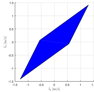
(f) Image of the RTS into the (\dot{i}_2, \dot{i}_3) -space
