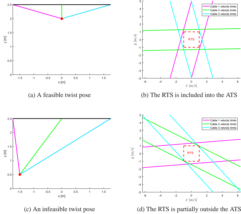
Fig. 5: A feasible twist pose and an infeasible twist pose of the CDPR
