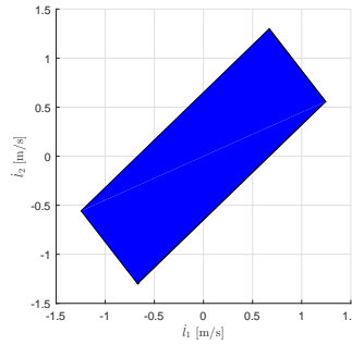
(d) Image of the RTS into the (\dot{i}_1, \dot{i}_2) -space
