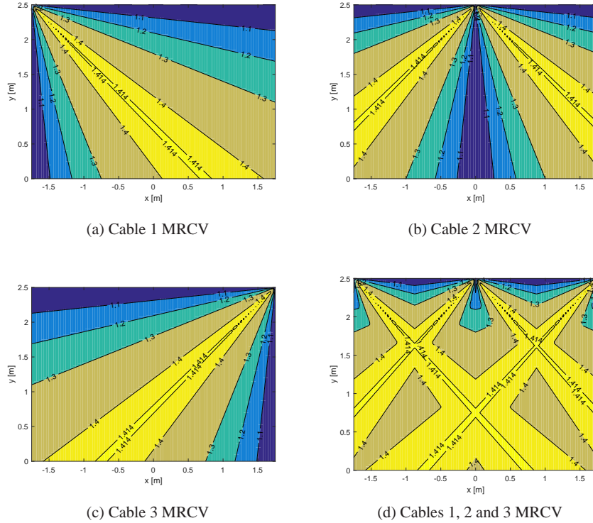
Fig. 4: Maximum Required Cable Velocity (MRCV) of each cable through the Cartesian space for the RTS shown in Fig. 3b
