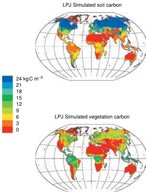
Fig. 9 LPJ-simulated global fields of vegetation and soil carbon (kg C m -2 ) for the modern climate.
