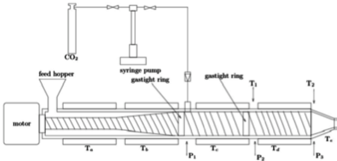
Figure 1: Experimental device
