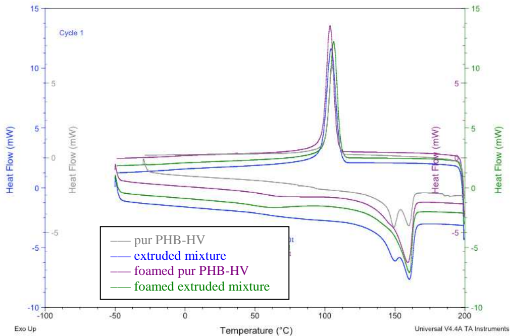
Figure 1. DSC spectra
