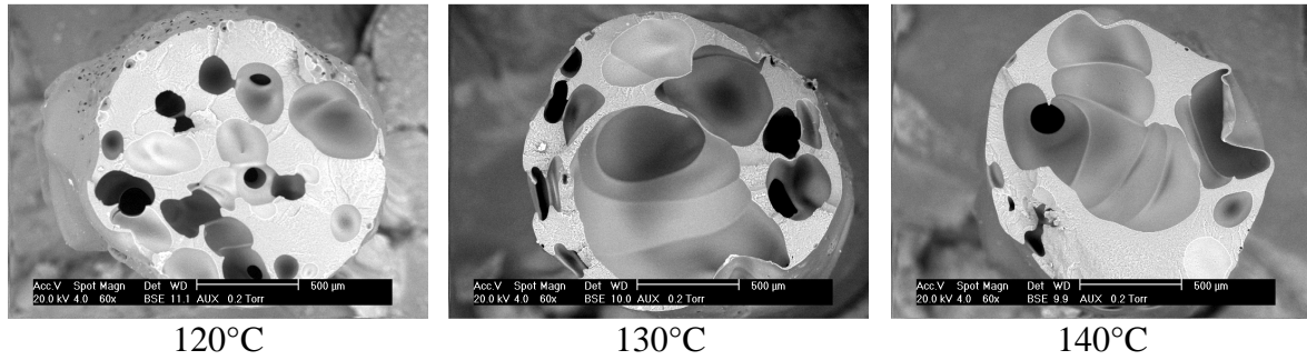
Figure 6. SEM pictures for series 1 at différent T_f
