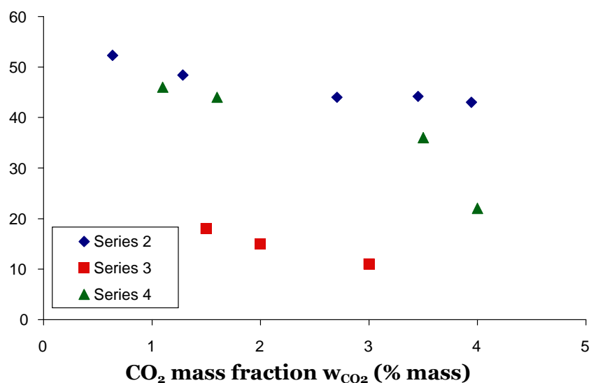
Figure 8. Evolution of the porosity \epsilon with the CO 2 mass fraction
