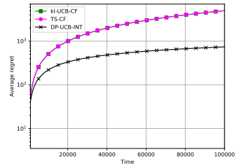
(c) Regret plots for \epsilon = 1 for kl-UCB-CF and TS-CF, DP-UCB-INT
