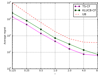
(b) Regret plots for kl-UCB-CF and TS-CF with T = 10^5 , \epsilon = \{\frac{1}{8}, \frac{1}{4}, \frac{1}{2}, 1, 2, 4, 8\}
