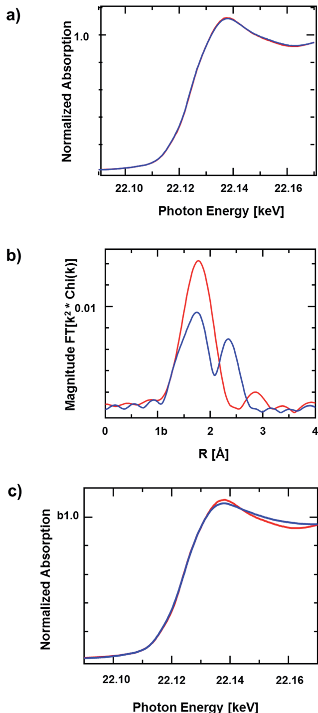
Fig. 13 (a) Ru K-edge XANES from 22.09 to 22.17 keV (red: Ru- \text{C}_{60} 1/1 \text{N}_2 at RT, and blue: Ru- \text{C}_{60} 1/1 \text{H}_2 at 150 °C); (b) magnitude of the Fourier transform of k^2 -weighted Ru EXAFS ( k^2: \Delta k = 2.8\text{--}11.3\text{ \AA}^{-1} ) (blue: Ru- \text{C}_{60} 2/1, \text{H}_2 at 150 °C, red: Ru- \text{C}_{60} 1/1, \text{H}_2 at 150 °C); and (c) Ru K-edge XANES from 22.09 to 22.17 keV (blue: Ru- \text{C}_{60} 1/1, \text{H}_2 at 150 °C red: Ru- \text{C}_{60} 2/1, \text{H}_2 at 150 °C).
