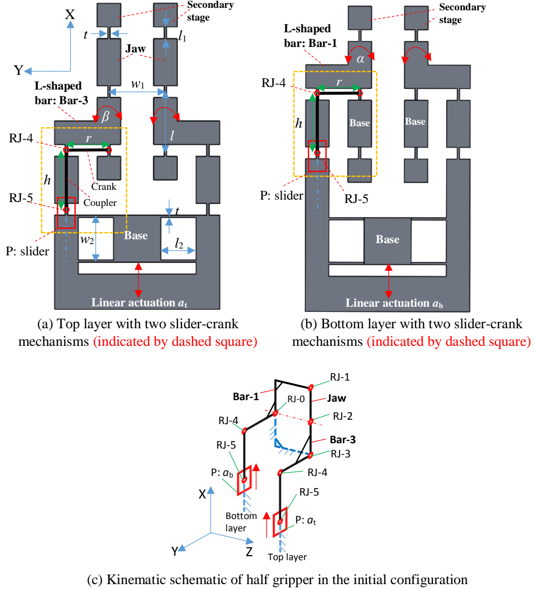
Figure 8: Design details of the multi-mode compliant gripper
