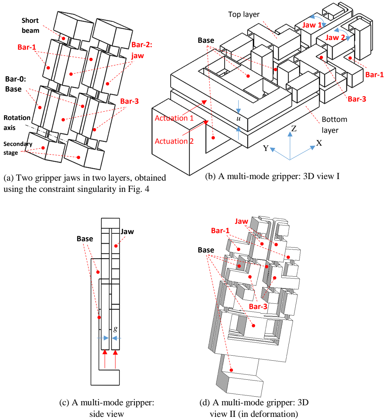
Figure 7: The synthesized multi-mode compliant gripper
