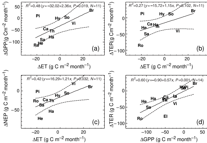
Fig. 6 Three correlation plots of year 2003 minus year 2002 differences of gross primary productivity ( \Delta GPP), ecosystem respiration ( \Delta TER) and net ecosystem productivity ( \Delta NEP) with respective evapotranspiration differences ( \Delta ET), and one plot with the correlation between \Delta TER and ( \Delta GPP). Anomalies are calculated for months July–September. Linear regression lines, 95% confidence bands and regression characteristics are indicated.
