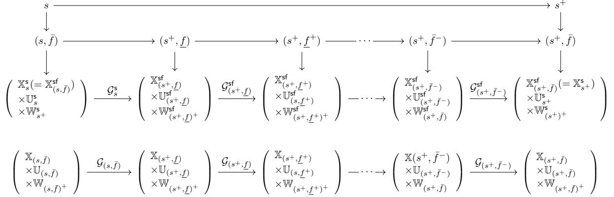
Figure 3: Original dynamics and their reformulation on the product timeline on the slow time interval [s, s^+ [= \{(s, \bar{f}), (s^+, \underline{f}), \dots, (s^+, \bar{f}^-)\}
