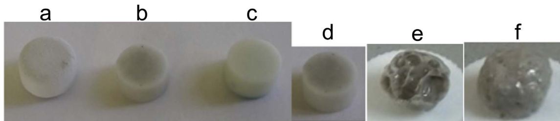
Fig. 4. Photographs of pellets made with glass powders a) without thermal treatment ( \varnothing 6 mm), and b) to f) after 2 h at 850 °C with respectively from the left to the right SG1, SG3, SG2, SS1 (bottom) and SS1 (top) pellets.
