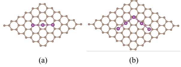
Fig. 1 (Color online) View of different adsorption sites of molecules (purple circles) on graphene layer (brown circles) : (a) triiodide and (b) pentaiodide adsorbed on (6 \times 6) and (7 \times 7) primitive cells of graphene layer respectively.
