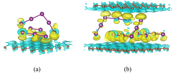
Fig. 2 (Color online) Charge density difference showing electron transfer between iodine molecules and (4 \times 4) graphene layer (a) and (4 \times 4) bilayer (b). Yellow represents positive electronic densities which accept electrons and cyan stands for negative densities which donate electrons.
