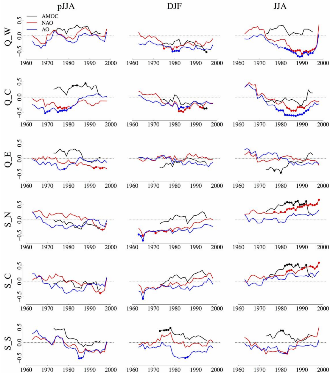
Fig. 9. Moving correlations between previous summer (pJJA; left-hand panels), winter (DJF; middle panels) and current summer (JJA; right-hand panels) large-scale indices, and the six regional chronologies (Q_W, Q_C, and Q_E in NA; and S_S, S_C and S_N in NE). Large-scale indices include AMOC (black), NAO (red), and AO (blue). Moving correlations were calculated using 21-yr windows moved one year at a time and are plotted using the central year of each window. Correlations were calculated over the 1961-2005 period for AMOC, and over the 1950-2008 period for NAO and AO. Windows of significant correlations ( P < 0.05 ) are marked with a dot.
