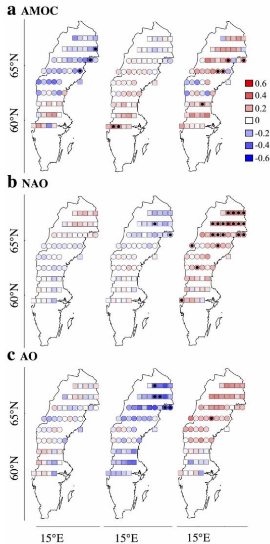
Fig. 8. Correlation between seasonal AMOC (a), NAO (b), and AO (c) indices, and growth patterns at the local level in Sweden. Seasonal indices were calculated as mean of monthly indices and include previous summer (left-hand panels), winter (middle panels), and current summer (right-hand panels). Correlations were calculated over the 1961-2005 period for AMOC, and over the 1950-2008 period for NAO and AO. To visualize the separation between regional clusters, correlation values at S_C grid cells are plotted with circles. Significant correlations ( P < 0.05 ) are marked with a black dot.
