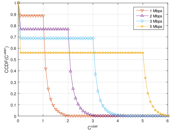
Fig. 6: CCDF of user capacity for 5:1 user to base station ratio, reuse factor \Delta = 1 , and different values of C^{req}
