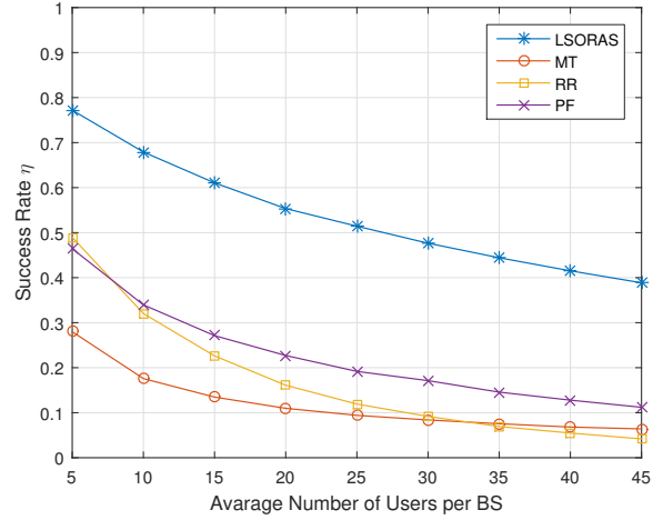
Fig. 4: Average SR vs the number of users for 100 BS in the service area with C^{req} = 2 Mbps and reuse factor \Delta = 1
