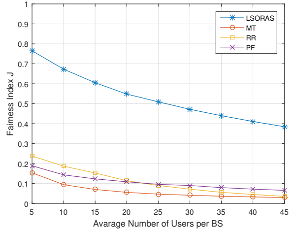
Fig. 5: Average fairness index as a function of number of users for 100 BS in the service area with C^{req} = 2 Mbps and frequency reuse factor \Delta = 1
