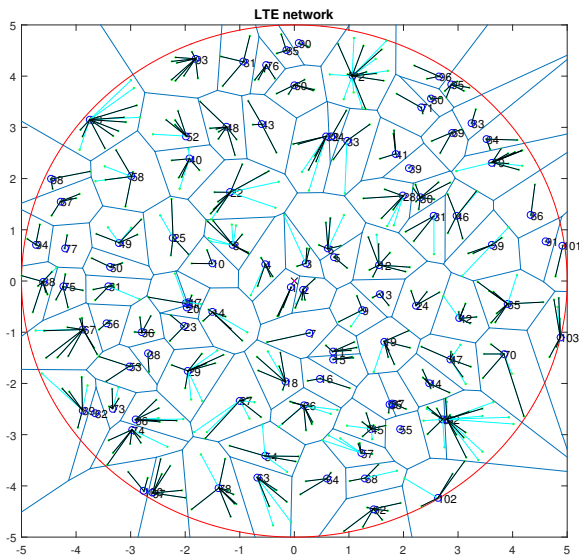
Fig. 1: Modeled broadband network with a PPP describing the position of BSs, users and cells
