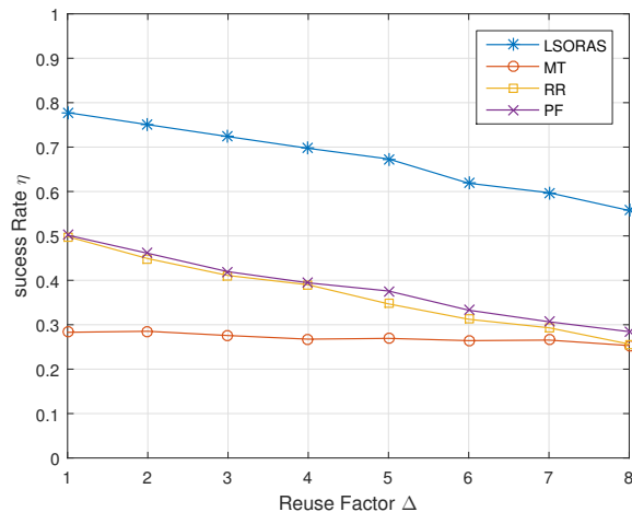
Fig. 8: Average success rate as a function of reuse factor \Delta with C^{req} = 2 Mbps and 5:1 user to BS ratio
