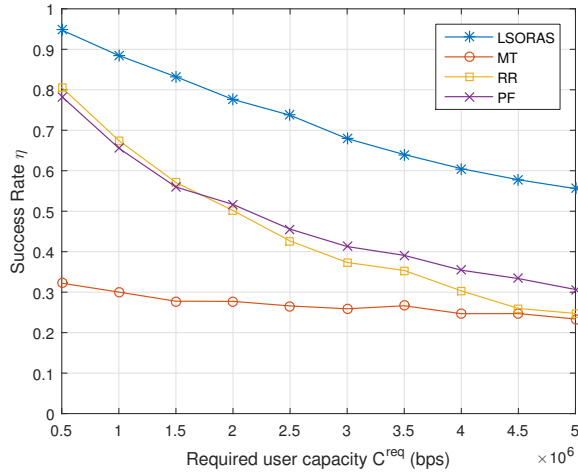
Fig. 7: Average success rate as a function of C^{req} , with 5:1 user to BS ratio, and reuse factor \Delta = 1
