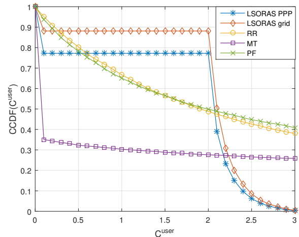
Fig. 2: CCDF of user capacity for 5:1 user to base station ratio, C^{req} = 2 Mbps and frequency reuse factor \Delta = 1
