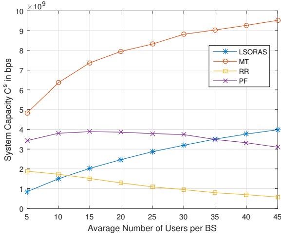
Fig. 3: Average system capacity as a function of number of users for 100 BS in the service area with C^{req} = 2 Mbps and frequency reuse factor \Delta = 1
