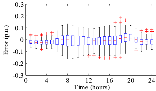
Fig. 9. Load prediction on 120 test days.
