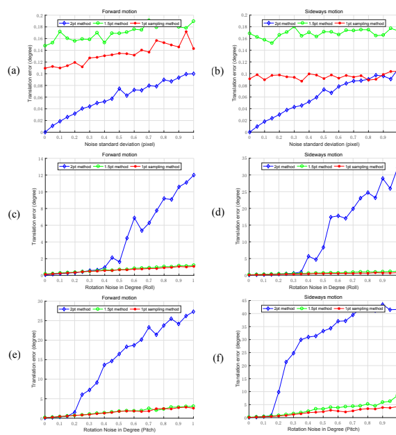
Fig. 2. Translation error with "PLANAR" setting: Evaluation of the 1.5pt linear solution method, 1pt method by sampling for x-z translation direction and 2pt method. Left: forward motion, right: sideways motion. (a) and (b) are with varying image noise. (c), (d), (e) and (f) are under different IMU noise and constant image noise 0.5 pixel standard deviation. (c) and (d) are with Roll angle noise. (e) and (f) are with Pitch angle noise.
