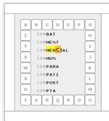
Figure 3. CentraList interface
