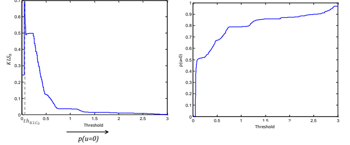
Fig. 3: Representation of KLS_0 and p(u=0) in function of the threshold value.
