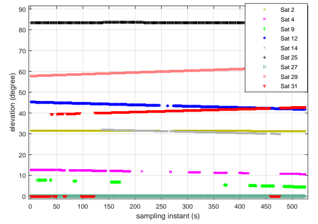
Fig. 14: The elevation of the satellites in view.
