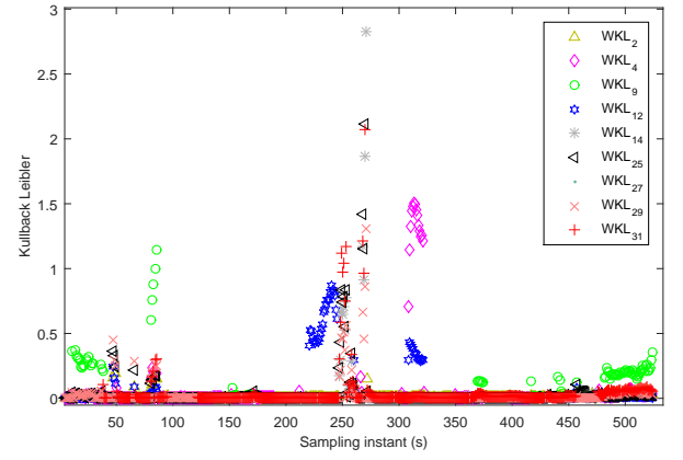
Fig. 13: The WKLi for the fault exclusion
