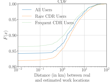
(b) Errors in Internet flow data: Work
