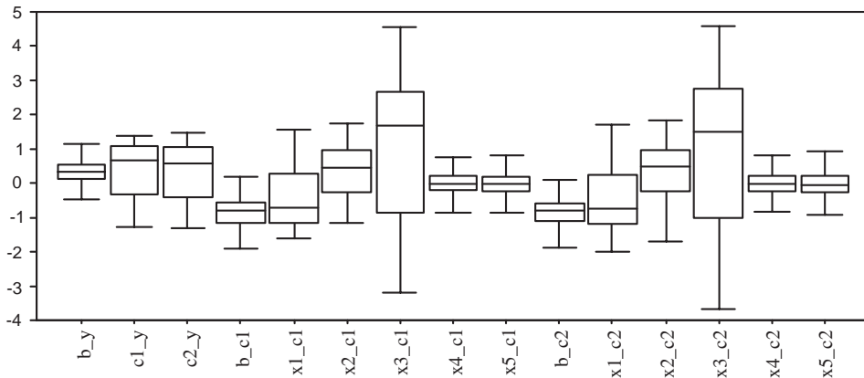
Fig. 11. Design 4: empirical distributions of the weight estimations ( n = 250 ).
