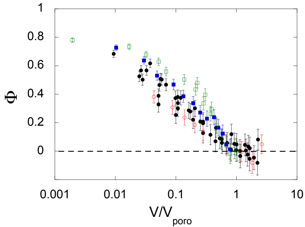
Figure 4: Reduced shift function \Phi = 1 - \Delta\Gamma/\Delta\Gamma^{(0)} with respect to the reduced velocity V/V_{poro} . Closed circles: c = 5\% , \phi = 0\% ; open circles: c = 5\% , \phi = 60\% ; closed squares: c = 10\% , \phi = 0\% ; open squares: c = 15\% , \phi = 0\% . The dashed line \Phi = 0 corresponds to the high velocity, undrained tip limit.
