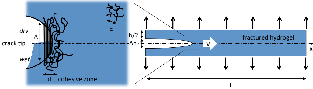
Figure 1: Right: Fracture setup. The gel sample of length L , initial height h and thickness e (not shown) is loaded (displacement \Delta h ) in pure shear configuration. The crack tip propagates at a velocity V along the x direction. Left : Schematic blow-up representation of the gel tip. In the cohesive zone of extension d along the fracture plane, the triple helix crosslinks (meshsize \xi ) are unzipped and the chains are extracted taut (contour length \Lambda ). In the “dry tip” configuration (upper half) the chains are exposed to air while in the wet tip” one (lower half) they remain hydrated by a solvent drop wetting the crack opening.
