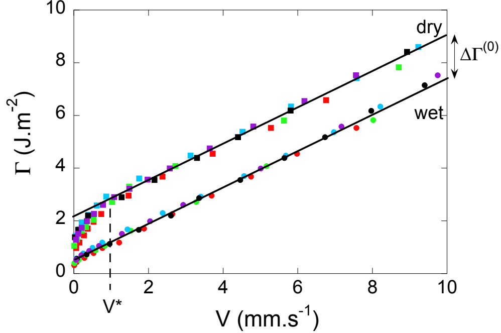
Figure 2: Fracture energy \Gamma with respect to the steady crack tip velocity V for five, nominally identical samples (different colors on line) in both the dry (squares) and wet (circles) crack tip configurations in a c = 5 wt.% \phi = 0 gel. The velocity V^* corresponds to the departure from linearity of the \Gamma_{dry}(V) curve. For V \gg V^* data are aligned on parallel straight lines shifted by \Delta\Gamma^{(0)} .
