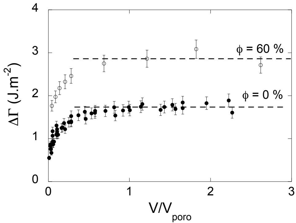
Figure 3: Shift function \Delta\Gamma = \Gamma_{dry} - \Gamma_{wet} plotted with respect to the reduced velocity V/V_{poro} for two gels with c = 5 wt.% differing by their glycerol content \phi . Dashed lines correspond to \Delta\Gamma^{(0)} (see Fig.2).
