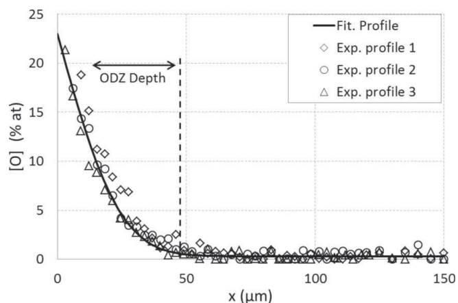
Figure 4 Experimental oxygen profiles (using EPMA) for sample A (873 K, 1000 h) and corresponding fitted profile.
