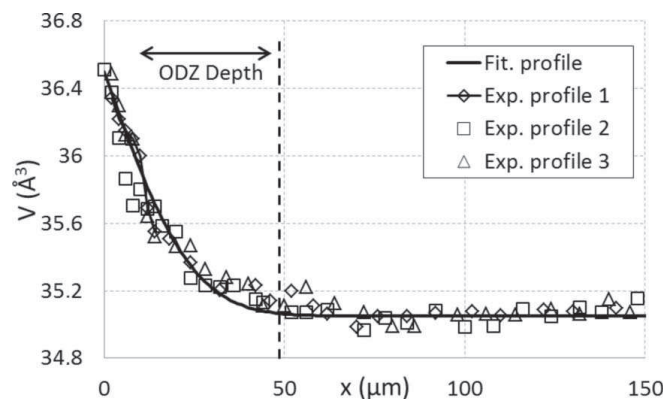
Figure 6 Experimental α-phase unit-cell volume profiles for sample A (873 K, 1000 h) and the corresponding calculated α-phase unit-cell volume profile.
