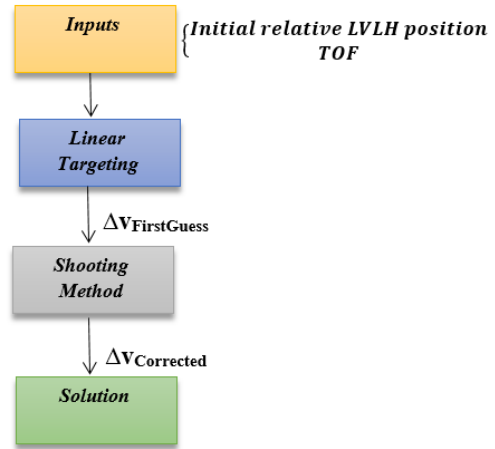
Figure 5. General Structure of the Algorithm
