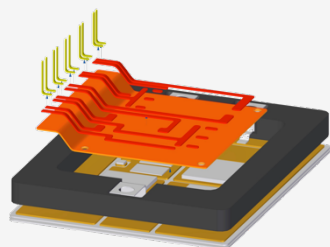
Flex-cover technology (Dynex)
