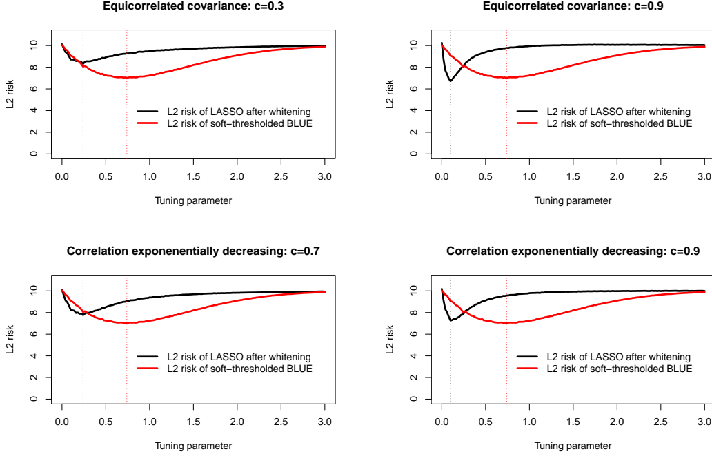
Figure 3. The x-axis and y-axis of these curves represent respectively the tuning parameter \lambda \geq 0 and the L_2 risk for both LASSO and soft-thresholded BLUE estimators. To obtain these curves we simulated 10000 the random vector Y and we computed the soft thresholded BLUE and LASSO estimator for \lambda \in \{0, 0.02, 0.04, \dots, 3\} . Computation of the LASSO estimator have been done with glmnet package [21]. In every cases, when \lambda = 0 these two functions are equal to \mathbb{E}(\|Y - \beta^*\|^2) and when \lambda is very large these two functions are approximately equal to \|\beta^*\|_2^2 . One can notice that the function \lambda \geq 0 \mapsto \mathbb{E}(\|\hat{\beta}^s(\lambda) - \beta^*\|^2) does not change in these four settings since, in each case, components of the BLUE have a \mathcal{N}(1, 1) marginal distribution. The minimum is 7.01 and is reached at \lambda = 0.74 . Depending on the setting, the minimum of the function \lambda \geq 0 \mapsto \mathbb{E}(\|\hat{\beta}^{\text{lasso},w}(\lambda) - \beta^*\|^2) is 8.30, 6.71, 7.76 and 7.25 is reached at \lambda = 0.24, \lambda = 0.10, \lambda = 0.24 and \lambda = 0.10 . Overall, after choosing properly the tuning parameter, one may notice that the L_2 risk is approximately equal or slightly smaller for the soft-thresholded BLUE than for the LASSO estimator.
