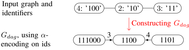
Fig. 4: Example of G_{dag} construction
