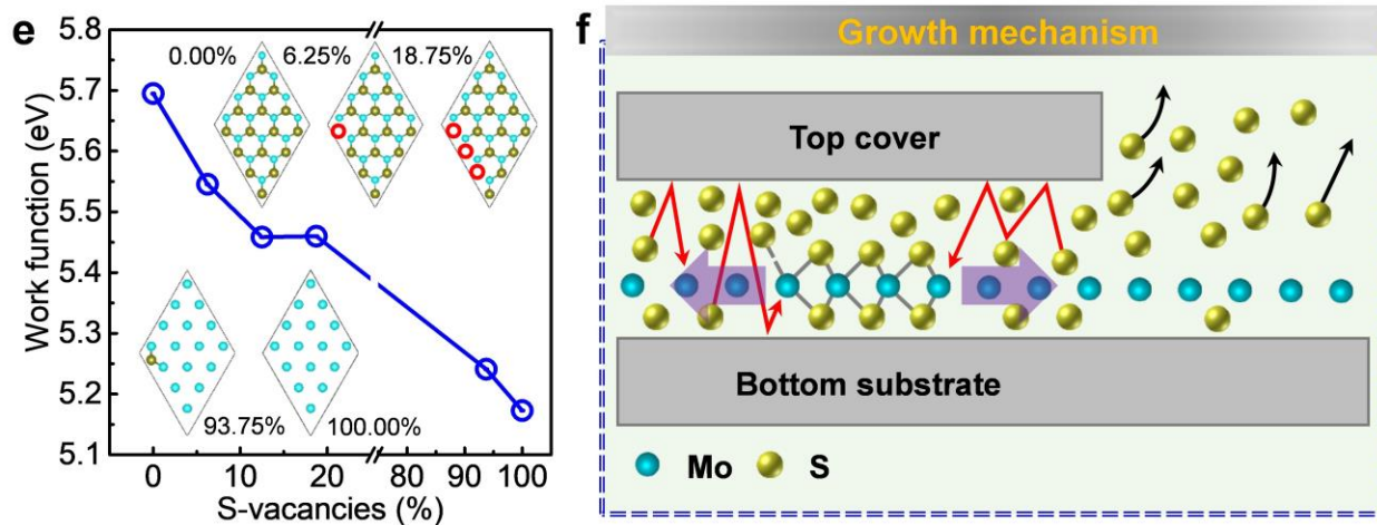
Figure 3. Solid-phase reaction growth mechanism of monolayer MoS 2 single crystal domains.
