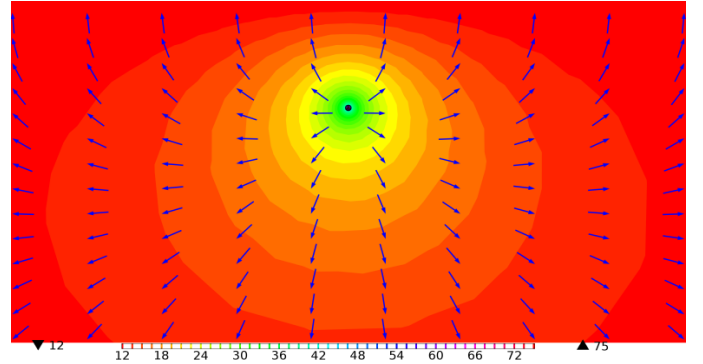
Fig. 10 Steady-state temperature field simulation ( ^{\circ}\text{C} ) of the cable environment. The blue arrows represent the heat flux.
