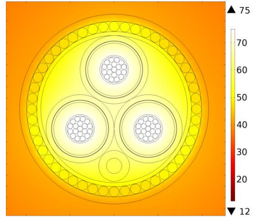
Fig. 9 Steady-state temperature field simulation ( ^{\circ}\text{C} ) of the submarine cable under normal load conditions.
