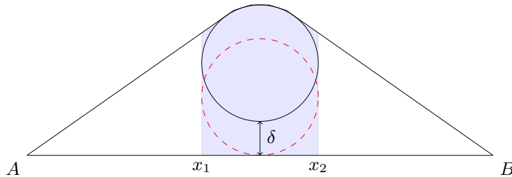
Figure 8: case where the diameter is realized by the only side [AB] of K^* which does not meet \mathcal{C} tangentially.
