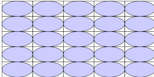
Figure 2: A packing with ellipses in a tiling with rectangles. It is intuitive that the density of this packing is equal to the ratio of the area of the ellipse over the area of the rectangle
