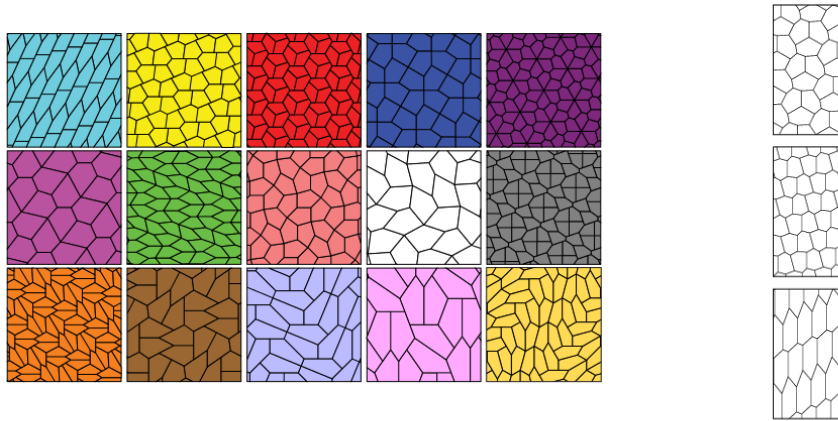
Figure 3: (Left) The fifteen kinds of tiling pentagons (Source https://commons.wikimedia.org/wiki/File:PentagonTilings15.svg ). (Right) The three kinds of tiling hexagon (Source http://mathworld.wolfram.com/HexagonTiling.html )
