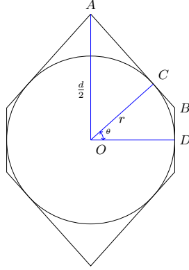
Figure 14: The hexagon H^{d,r}
