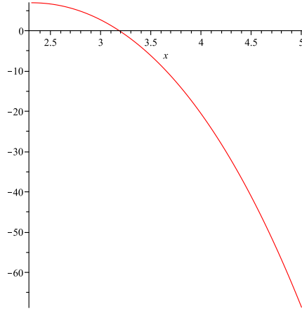
Figure 13: Plot of the function X \mapsto \sqrt{X^2 - 4}(14 - 5X^2) + 4X(X^2 - 3) .
