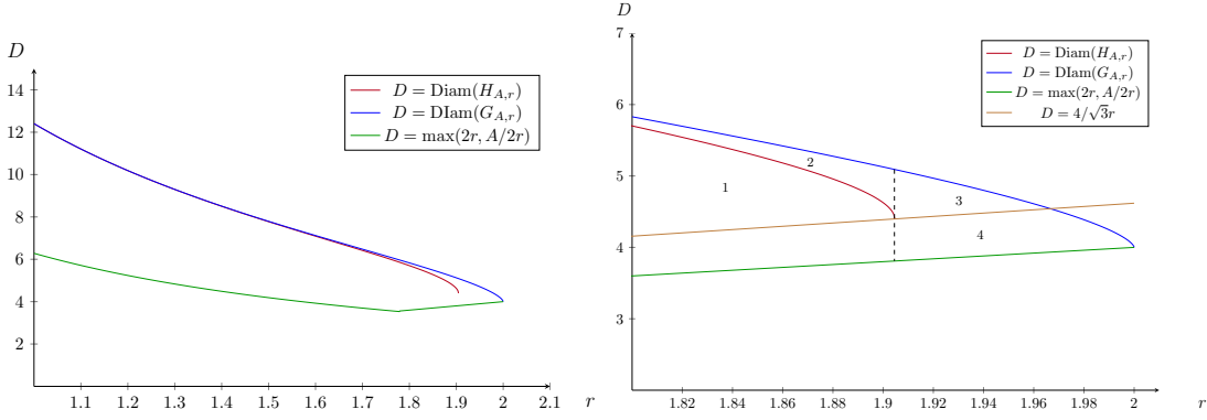
Figure 12: Left: Blaschke Diagram for (r(K), \text{Diam}(K)) under the condition |K| = 4\pi . Right: zoom on the right part of the diagram.
