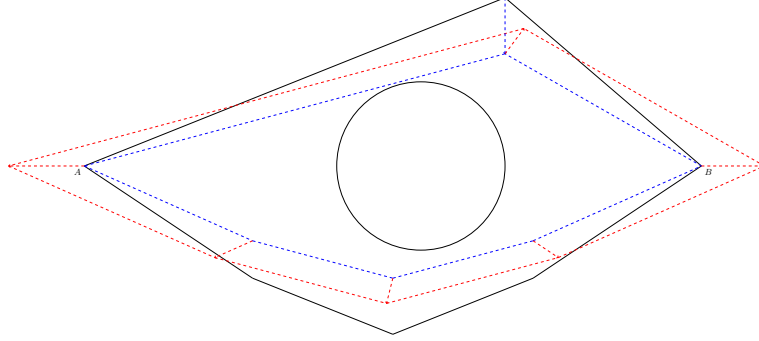
Figure 6: Illustration of the proof of Lemma 2: the hexagon K^* (black), the hexagon \rho_t(K^*) (blue) and the hexagon K_t (red).
