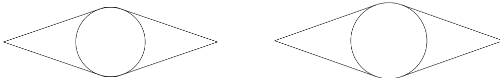
Figure 5: Left: the hexagon H_{A,r} and its inscribed circle. Right: the symmetric 2-cap body G^{D,r} and its inscribed circle.
