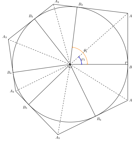
Figure 9: Parametrization of hexagons
