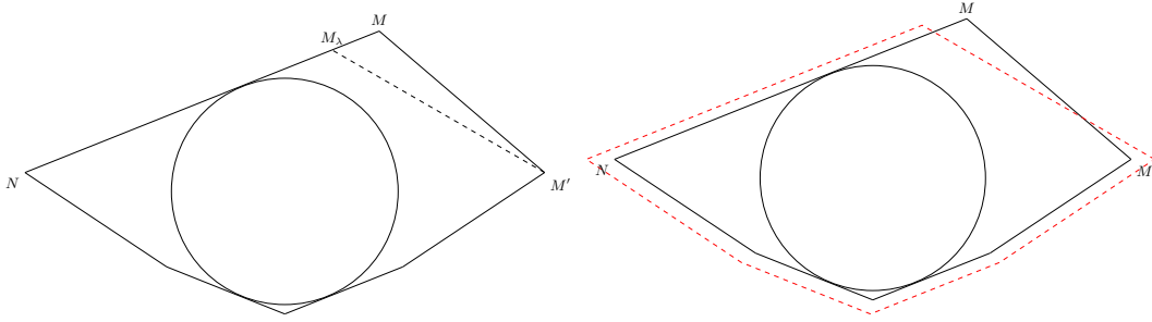
Figure 7: Geometrical illustration of the method: construction of \tilde{K} (left) and construction of \hat{K} (dotted line) from \tilde{K} (right).
