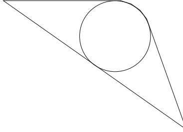
Figure 10: Hexagon maximizing D_{1,2}(\Phi) for A = 4\sqrt{3}
