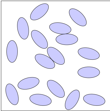
Figure 1: An example of a packing with ellipses, we can see the density as the ratio between the blue area and the entire square
