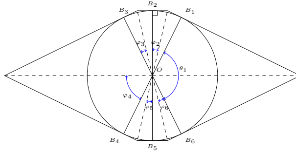
Figure 4: The p -hexagon H_{A,r} and its inscribed circle.
