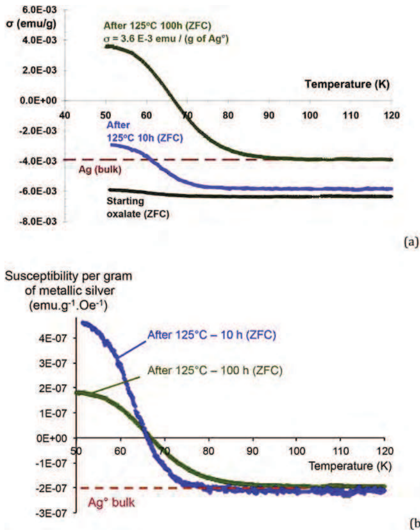
Fig. 5. (a) Zero field cooled magnetization under 20 kOe at different temperatures, for an oxalate sample at the early beginning of the decomposition, after 10 h and 100 h at 125 °C. The heat treatments were carried out inside the vibrating sample magnetometer to avoid contamination. The magnetization is divided by the sample mass measured after heat treatment. The magnetization under 20 kOe for diamagnetic bulk silver is given for comparison. (b) Susceptibility per gram of metallic silver formed after heat treatment, versus measurement temperature. The susceptibility of bulk silver is given for comparison.
