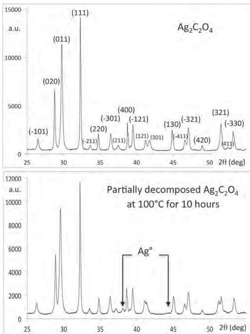
Fig. 2. X-ray diffraction patterns of pure silver oxalate and after its partial decomposition at 100^\circ\text{C} for 10 h.
