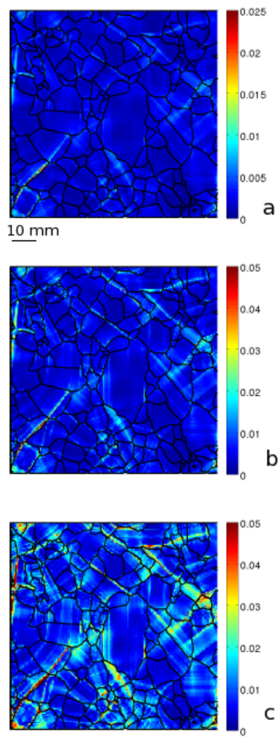
Figure 20: Evolution of the FFT-simulated equivalent strain field during the transient creep of a "2D-1/2" sample of ice, after (a) 0.15%, (b) 0.35% and (c) 0.60% compressive strain (see Grennerat et al. (2012)).
