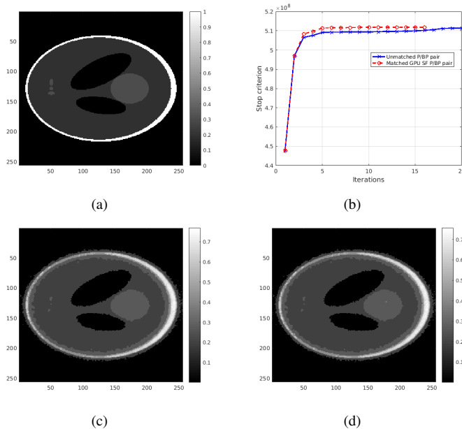
Fig. 1: Reconstruction of Shepp-Logan phantom (a) by the same MBIR method [7], with unmatched P/BP pair (c) and proposed matched GPU SF pair (d). Convergences are shown in (b).
