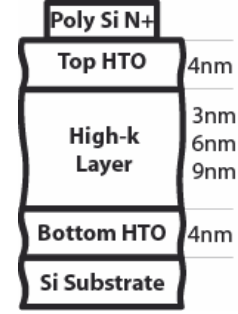
Fig. 1: Schematic showing the capacitor device stack studied in this work. Various high-k were investigated: \text{HfO}_2 , \text{Al}_2\text{O}_3 and HfAlO with different Hf:Al ratios (9:1, 1:4 and 1:9).
