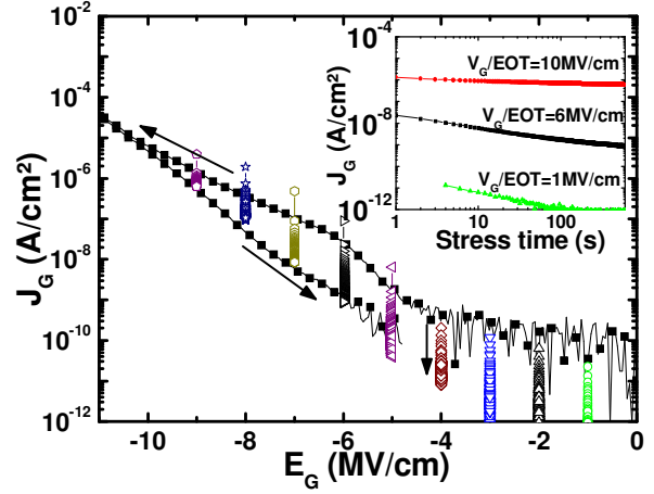
Fig. 3: Current density J_G versus equivalent electric field E_G of HTO /HfAlO 9:1 – 9nm/HTO stack. J_G -time measurements on virgin devices are also represented for different electric fields. Inset: J_G -time measurements performed at different applied electric field (1MV/cm, 6MV/cm and 10MV/cm) as a function of time.
