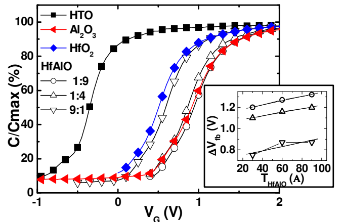
Fig. 2: C - V_G characteristics (in the virgin state) of OHO stacks with various high-k materials ( \text{Al}_2\text{O}_3 , \text{HfO}_2 and HfAlO with different compositions) compared to a 10nm HTO reference device. Inset: Flatband voltage shifts as a function of the HfAlO physical thickness.
