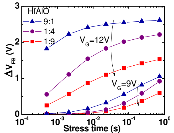
Fig. 4: Programming characteristics of OHO samples with various HfAlO compositions. The HfAlO thickness is 6nm.
